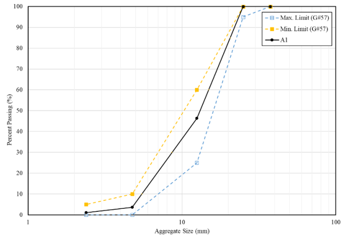
Figure 1. Gradation and size limits for A01 aggregate.
