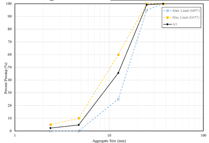
Figure 1. Gradation and size limits for A03 aggregate.
