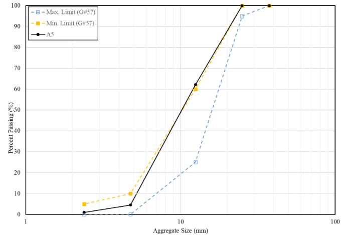
Figure 1. Gradation and size limits for A05 aggregate.
