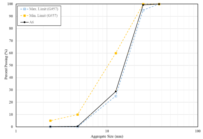
Figure 1. Gradation and size limits for A06 aggregate.
