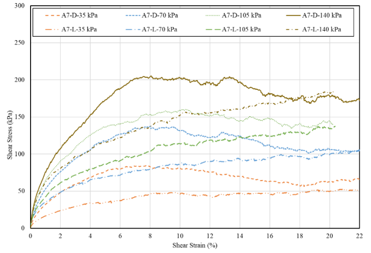
Figure 4. Shear strain versus shear stress relationship.
