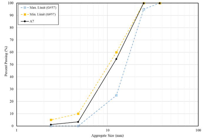
Figure 1. Gradation and size limits for A07 aggregate.
