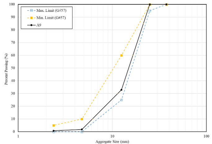
Figure 1. Gradation and size limits for A09 aggregate.
