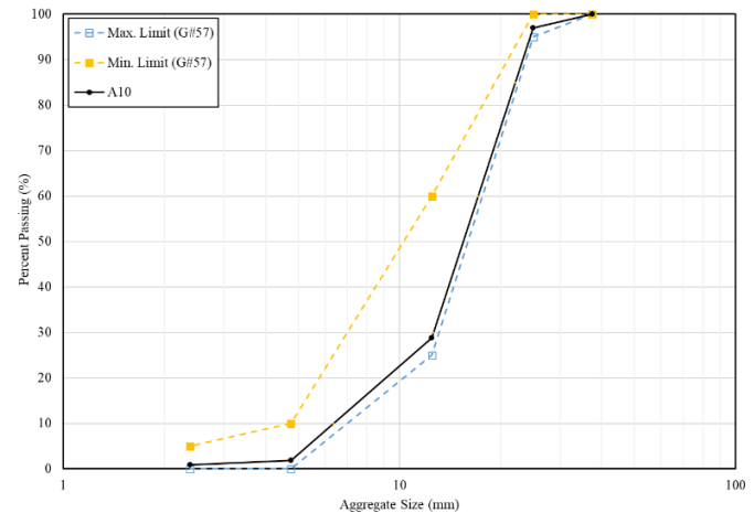
Figure 1. Gradation and size limits for A10 aggregate.
