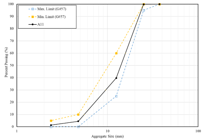
Figure 1. Gradation and size limits for A11 aggregate.
