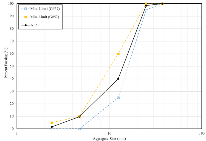
Figure 1. Gradation and size limits for A12 aggregate.
