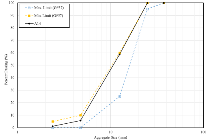
Figure 1. Gradation and size limits for A14 aggregate.
