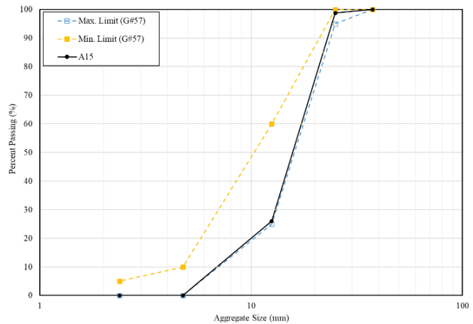
Figure 1. Gradation and size limits for A15 aggregate.
