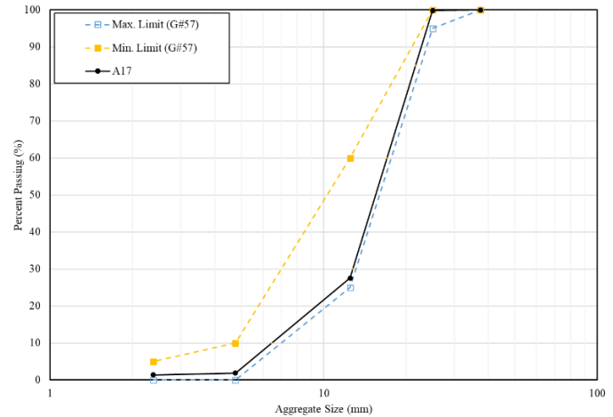
Figure 1. Gradation and size limits for A17 aggregate.
