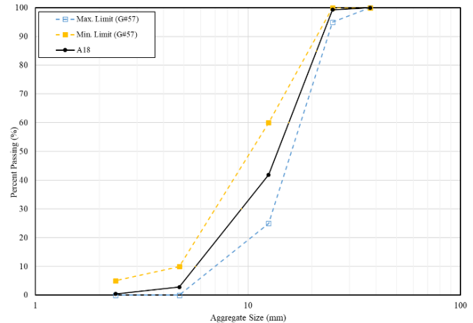
Figure 1. Gradation and size limits for A18 aggregate.
