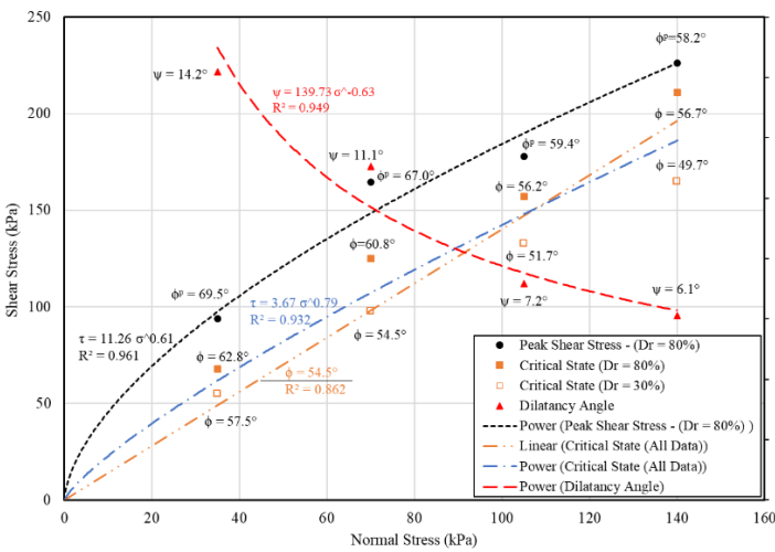
Figure 5. Linear and nonlinear Mohr Coulomb envelopes.
