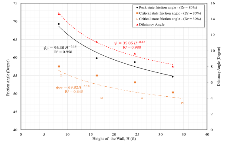
Figure 6. Friction and dilatancy angles versus wall height.
