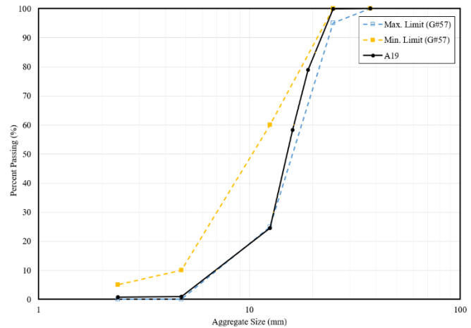
Figure 1. Gradation and size limits for A19 aggregate.
