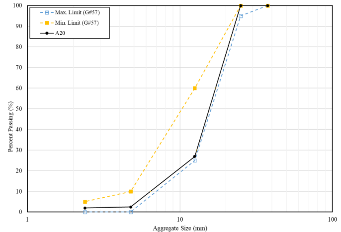
Figure 1. Gradation and size limits for A20 aggregate.
