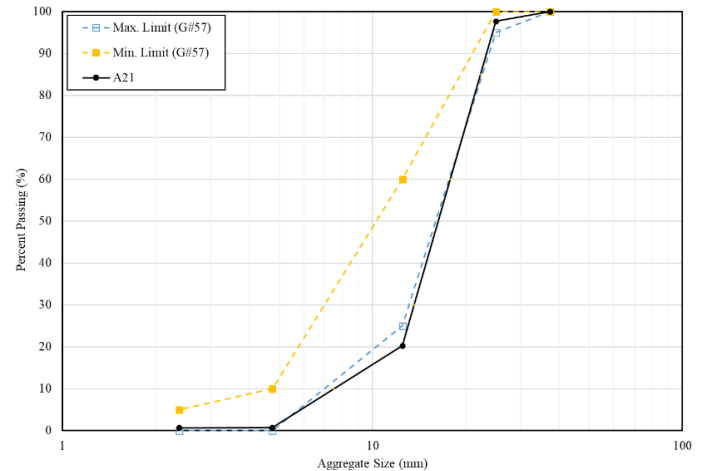
Figure 1. Gradation and size limits for A21 aggregate.
