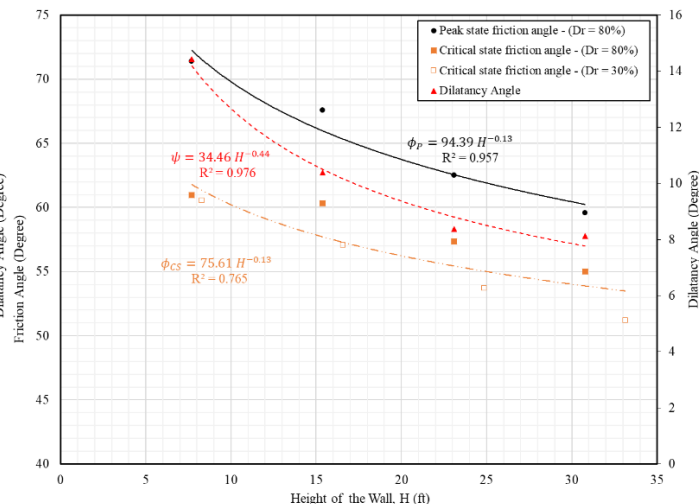
Figure 6. Friction and dilatancy angles versus wall height.
