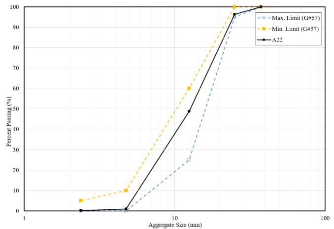
Figure 1. Gradation and size limits for A22 aggregate.
