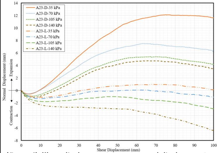
Figure 3. Shear displacement versus normal displacement.
