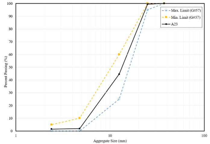
Figure 1. Gradation and size limits for A23 aggregate.
