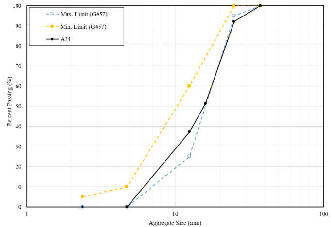
Figure 1. Gradation and size limits for A24 aggregate.
