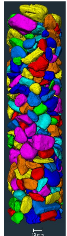
Figure 2. CT of aggregates.
