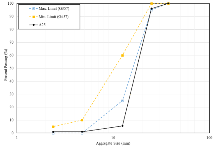
Figure 1. Gradation and size limits for A25 aggregate.
