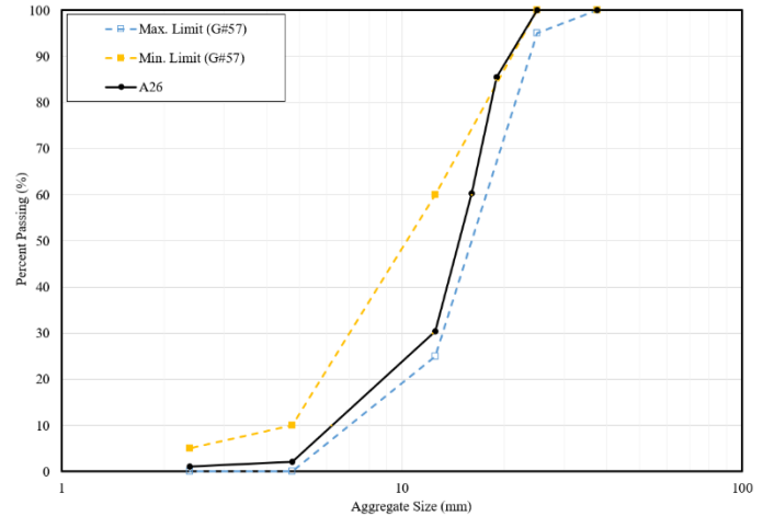
Figure 1. Gradation and size limits for A26 aggregate.
